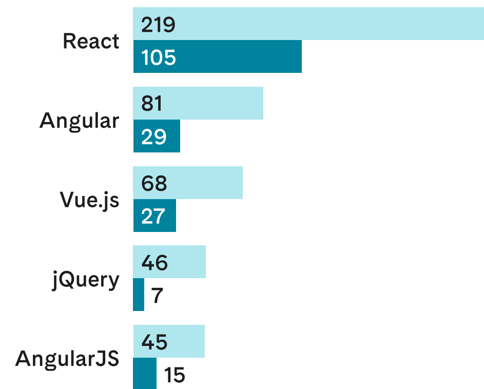
PRIMARY USED FRONTEND TECHNOLOGIES*
